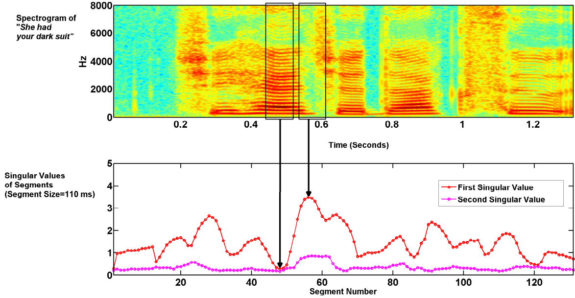
Figure 4: Figure showing speech spectrogram of “ She had your dark suit ” (top) and the corresponding first two singular values of covariances (bottom). Here, the covariance is computed for 110 ms sliding window ( i.e. , number of frame, N = 11 for window size 20 ms with an overlap of 50%) in temporal domain. The figure shows that portions of the speech segment with “stable” spectral information have lower eigenvalue where as regions with “highly varying” speech information correspond to higher singular values.
