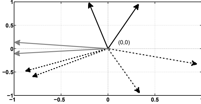
Figure 3: Graph of eigenvectors corresponding to the highest eigenvalues of local covariance matrices for four different speakers (in separate line styles). The data corresponds to the same phoneme /ae/ from SA2 sentences (“Don’t ask me to carry an oily rag like that”) in TIMIT corpus. For each speaker, two separate instances of the same sound are shown with identical line styles.
