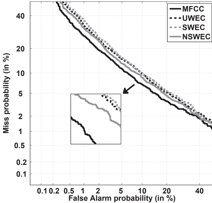
Figure 5: DET plot showing speaker verification performance on NIST SRE 2001 for 57-dimensional MFCC (static+ \Delta + \Delta\Delta ) and three 57-dimensional proposed features computed from first three eigenvectors using temporal window of 100 ms.
