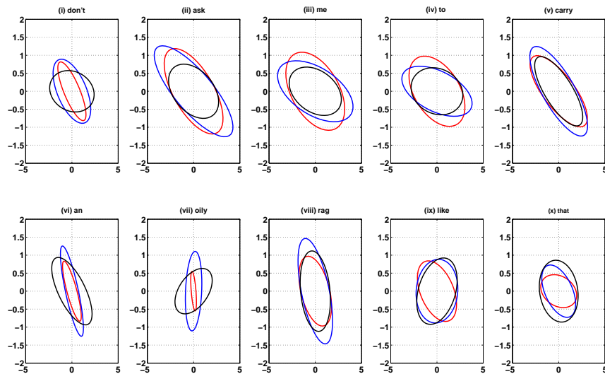
Figure 2: Plot of covariance matrices of three different female speakers corresponding to different words of SA2 sentences (“Don’t ask me to carry an oily rag like that”) in TIMIT corpus. First two dimensions of feature vector are chosen for this visualization.
