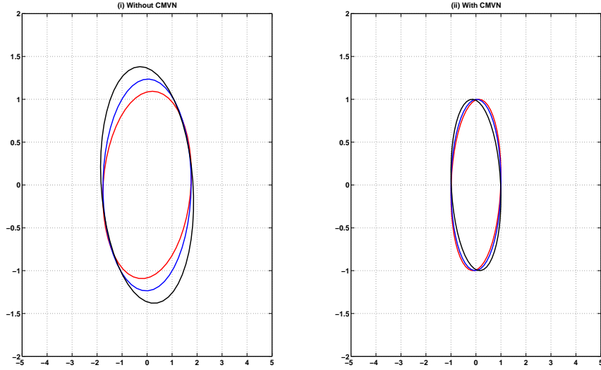
Figure 1: Plot of global covariance matrices of three different speakers of NIST SRE for (i) without CMVN and (ii) with CMVN processing. First two dimensions of feature vector are chosen for this visualization.
