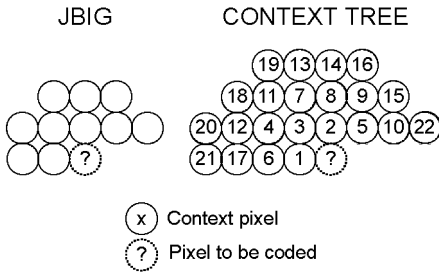
Fig. 2. The default three-line context template of the sequential JBIG (left), and the 22-pixel ordered neighborhood used for the context tree (right). The first 10 pixels in the neighborhood constitute the JBIG template.
